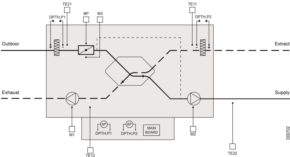
CX3010R/CX3020R, top view
