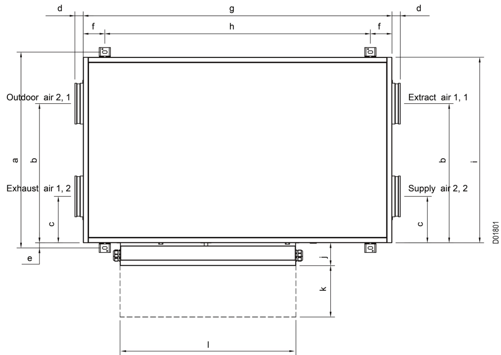
Top view: CX3010L/ CX3020L
