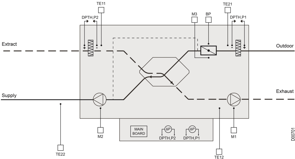
CX3010L/CX3020L, top view
